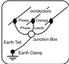
3 Phase with Junction Box
